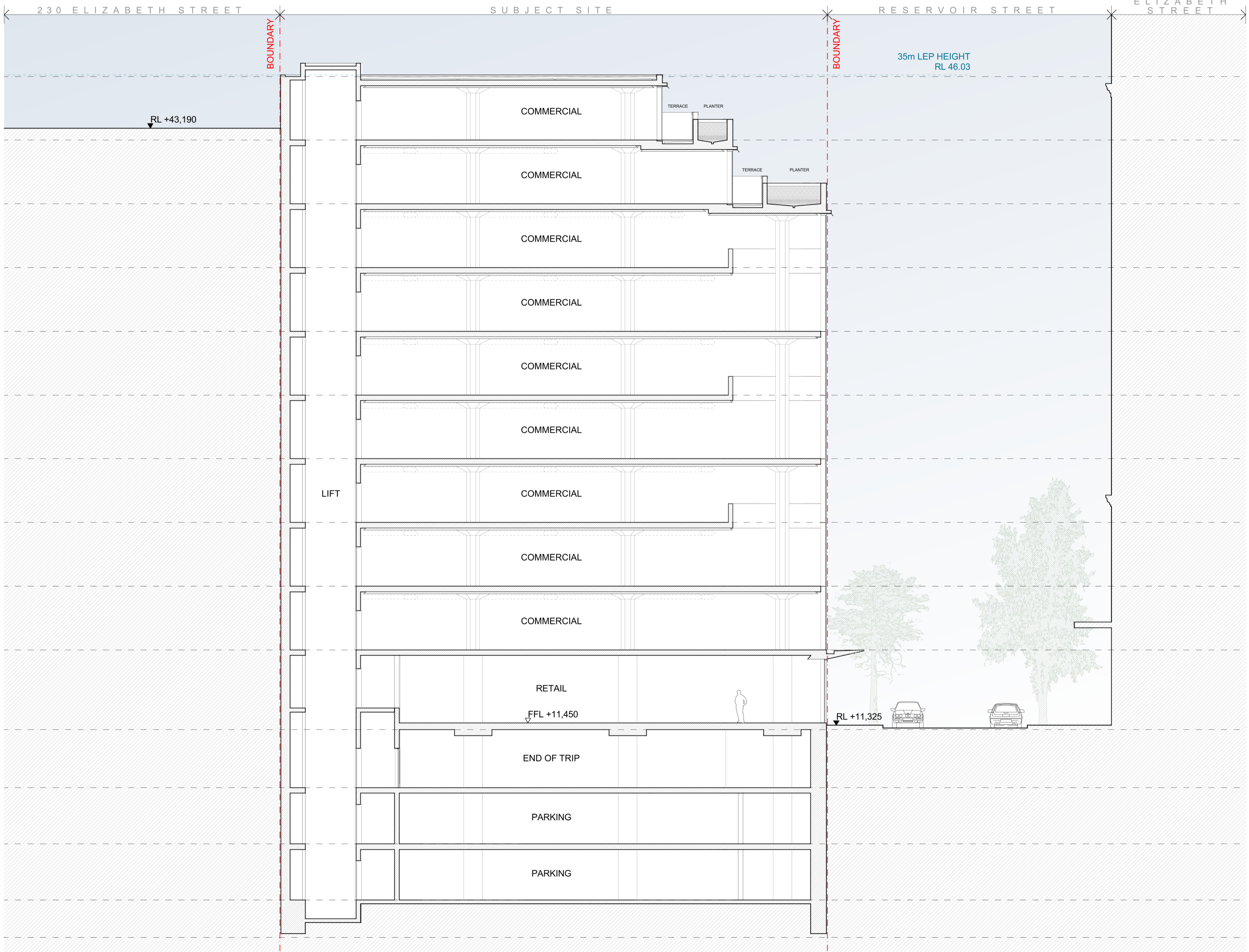
SECTION A 1:100
